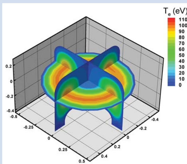
This partial-drive simulation, part of a simulation of the evolution of conditions inside the spheromak, shows that peak temperature of 98.8 eV occurring at 1 millisecond into the simulation.
